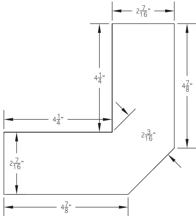
QuickLiner TS Outside Corner - Top View
